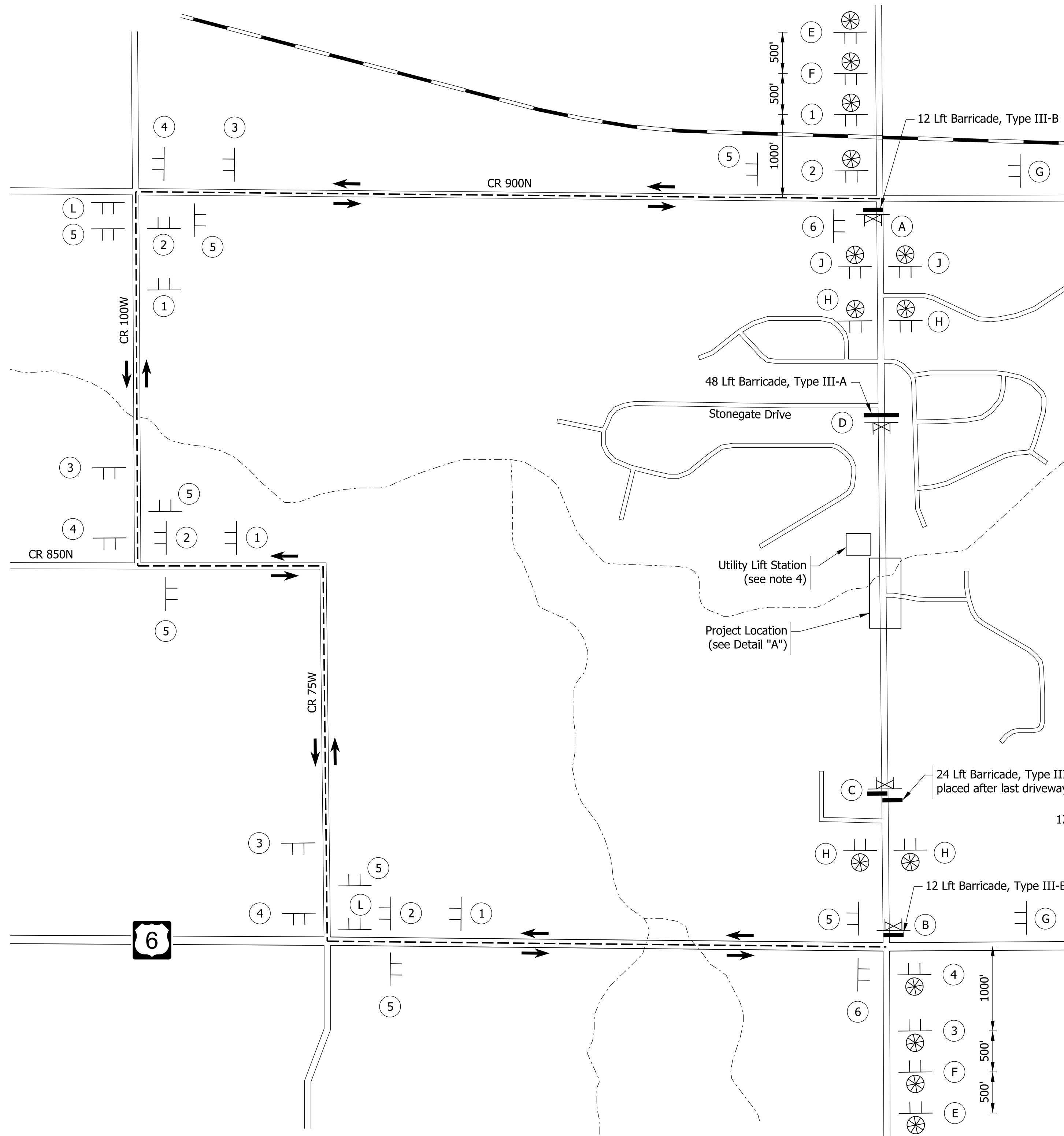
MAINTENANCE OF TRAFFIC DETOUR PLAN Scale: 1" = 500'
